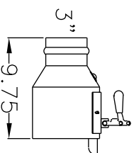
3"Ø OVAL TAILPIPE CONNECTOR WITH TOGGLE CLAMP AND CO2 PORT Fits over cuffed end of 3" hose (2TL0-9005)
