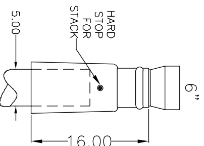
5" RUBBER DIESEL STACK CONNECTOR Includes swivel transition to 6" hose and 6" hose clamp (2TL0-9007)
